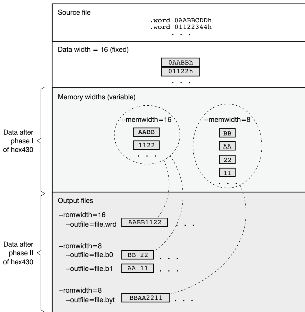
Figure 11-4. Data, Memory, and ROM Widths
